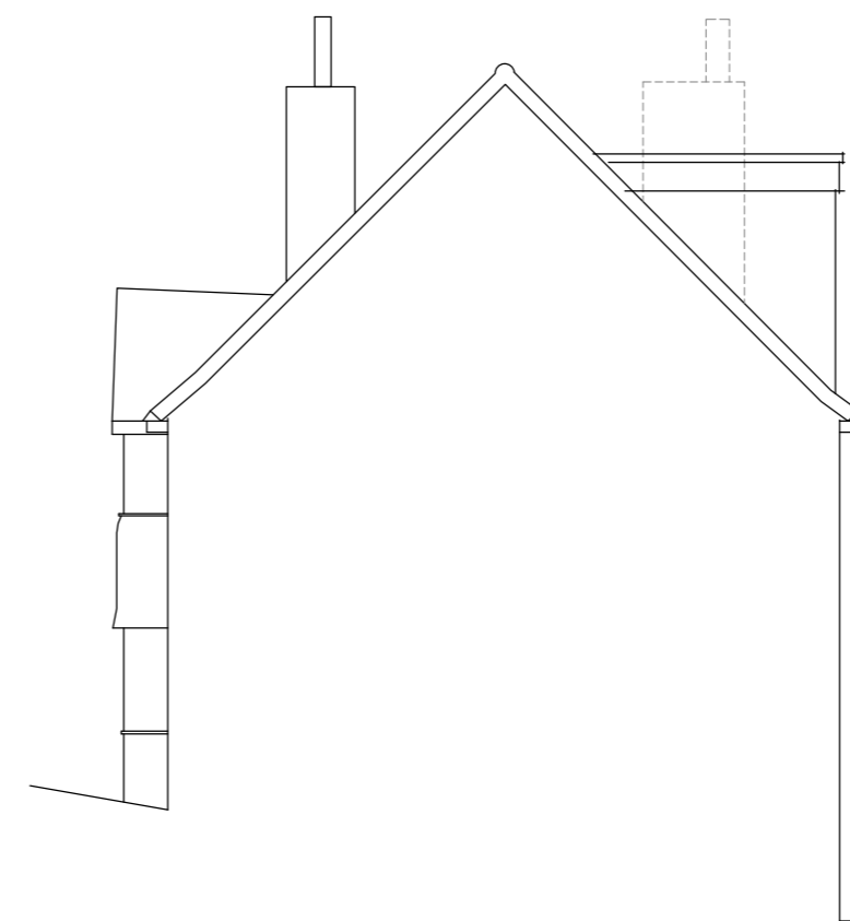
39 PEWLEY ROAD - HIDDEN ELEVATION
