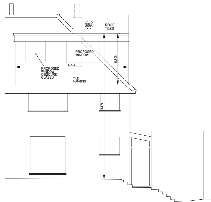
39 PEWLEY ROAD - ELEVATION-3
