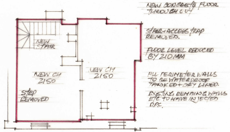
BASEMENT AS PROPOSED
