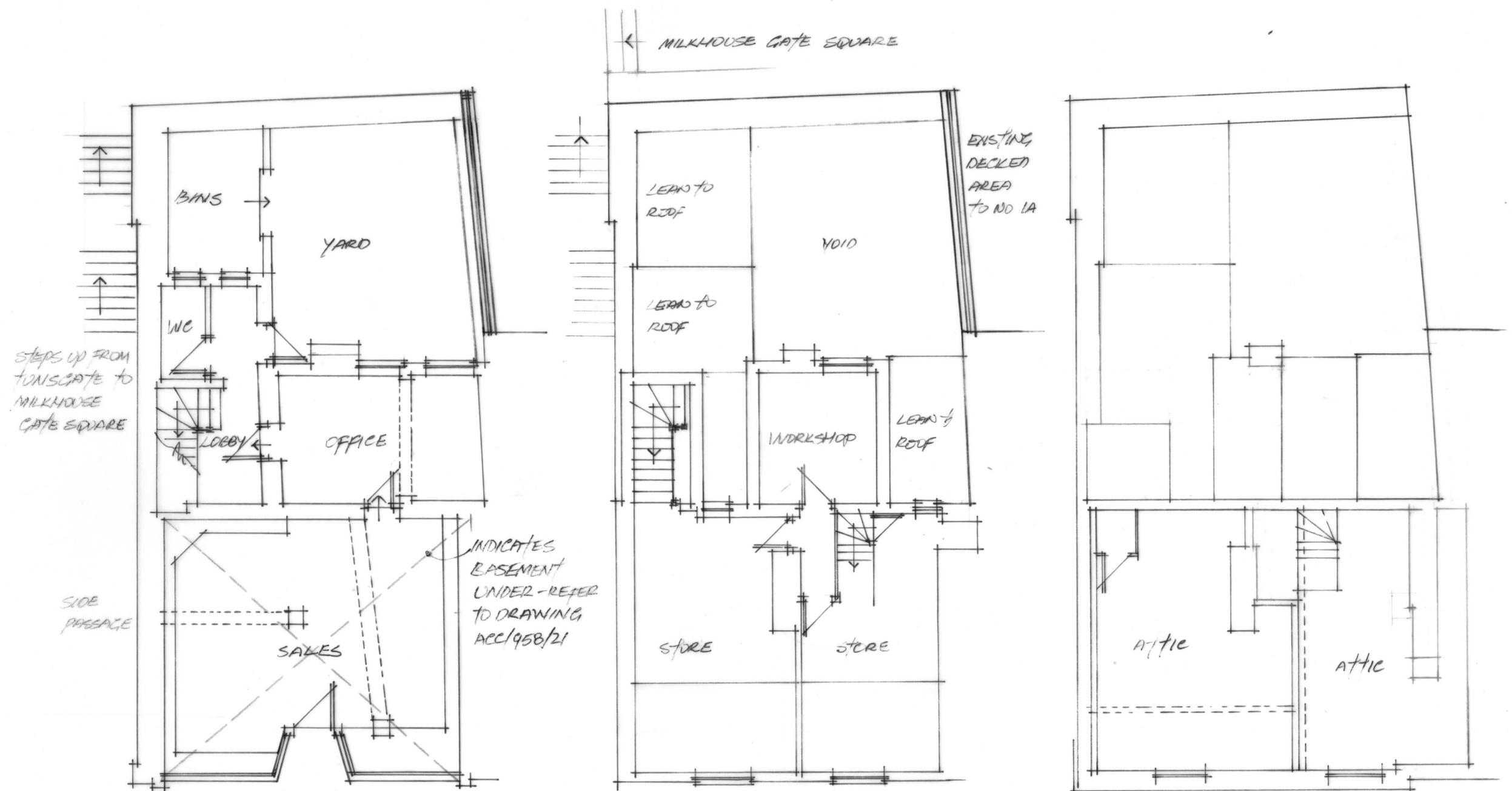
FIRST FLOOR
