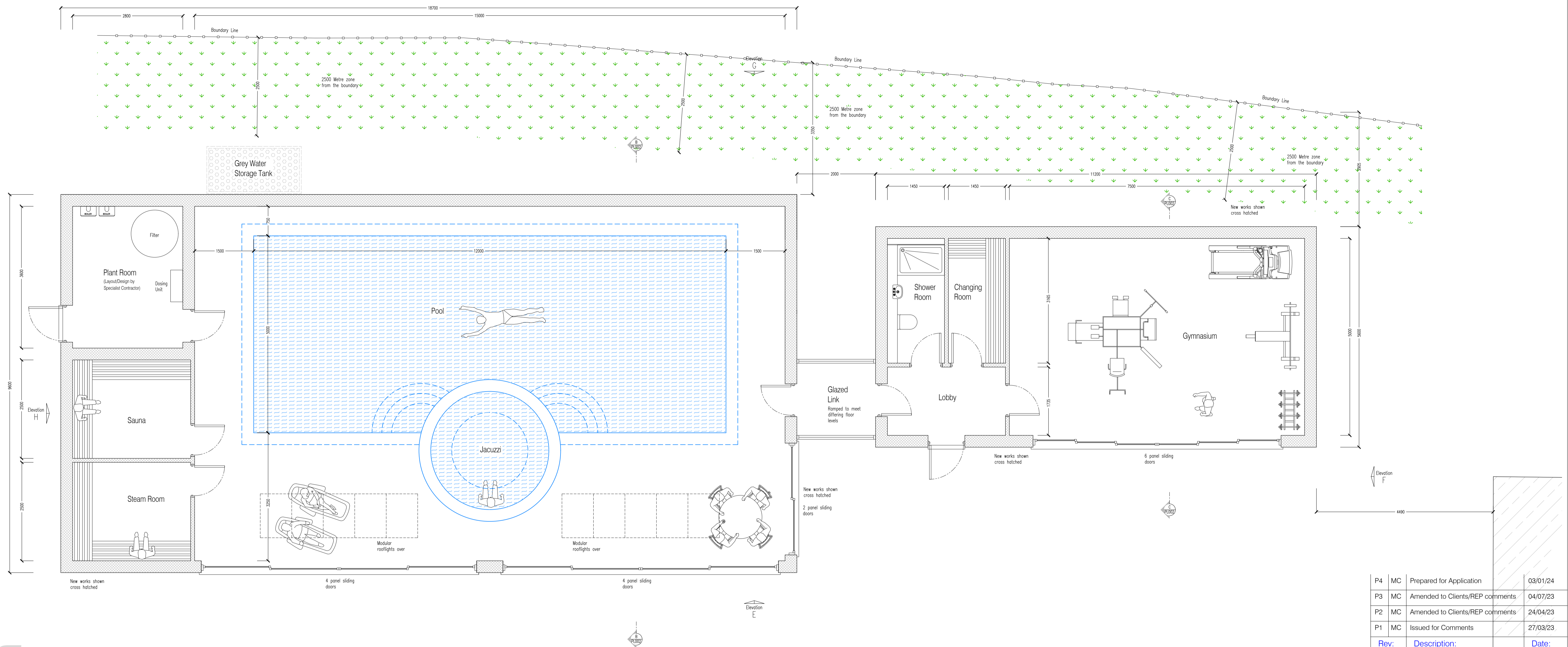
Proposed Pool/Gymnasium Floor Plan 1:50 Additional floor area created 220m 2
