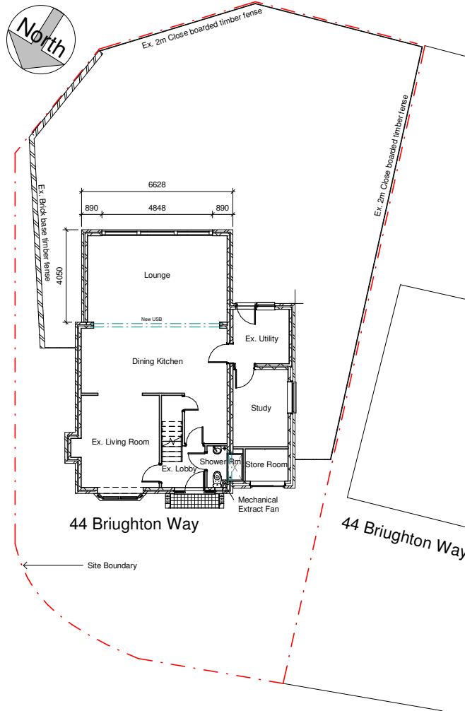
2 Proposed Site and Ground Floor Plan 1 : 100
