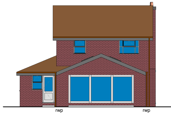
1 Proposed Front Elevation 1 : 100
