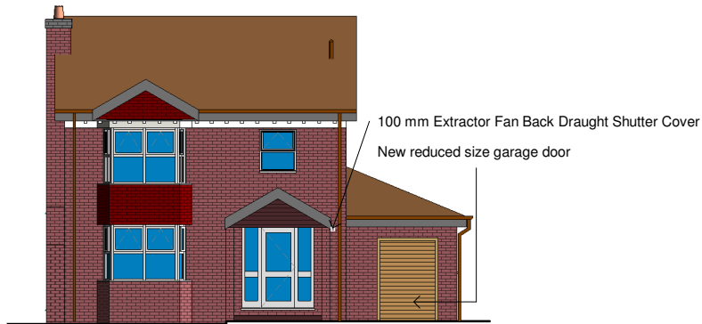
1 Proposed Front Elevation 1 : 100
