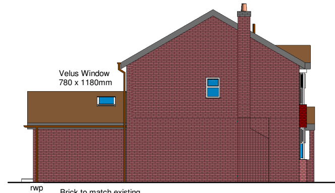
2 Proposed Side Elevation 1 : 100
