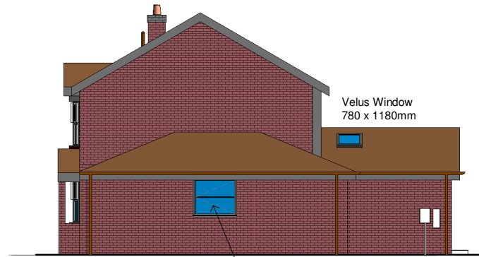
2 Proposed Side Elevation 1 : 100
