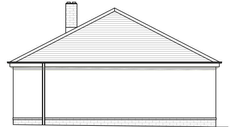
Existing Side Elevation-1
