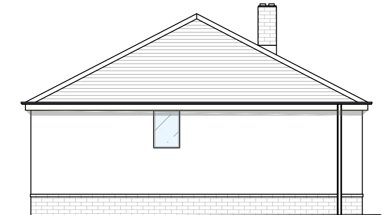
Existing Side Elevation-2
