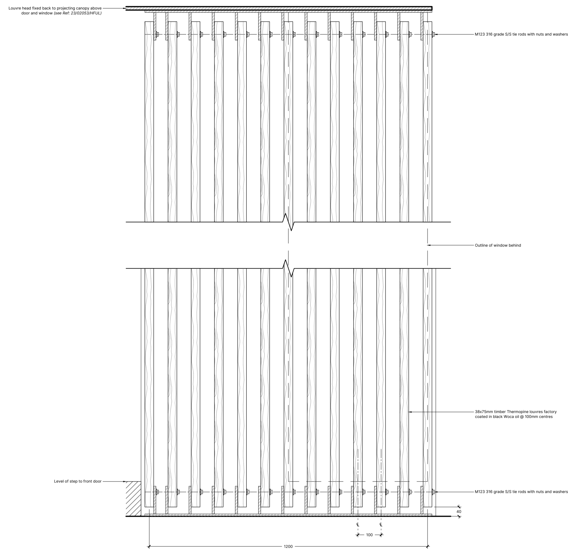
01 Detail Proposed Timber Louvres
