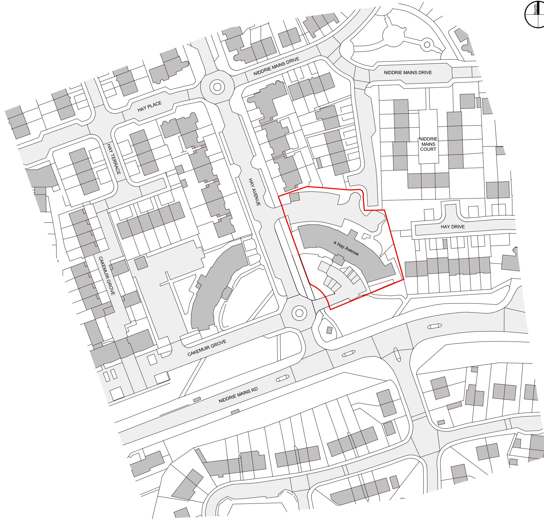
XX-Site - Location Plan 1 : 1250
