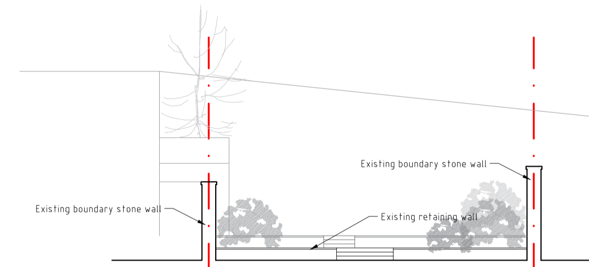
05 South East Elevation As Existing 1:100 @ A1
