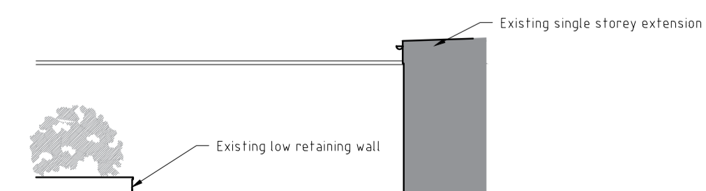
06 South West Elevation As Existing 1:100 @ A1
