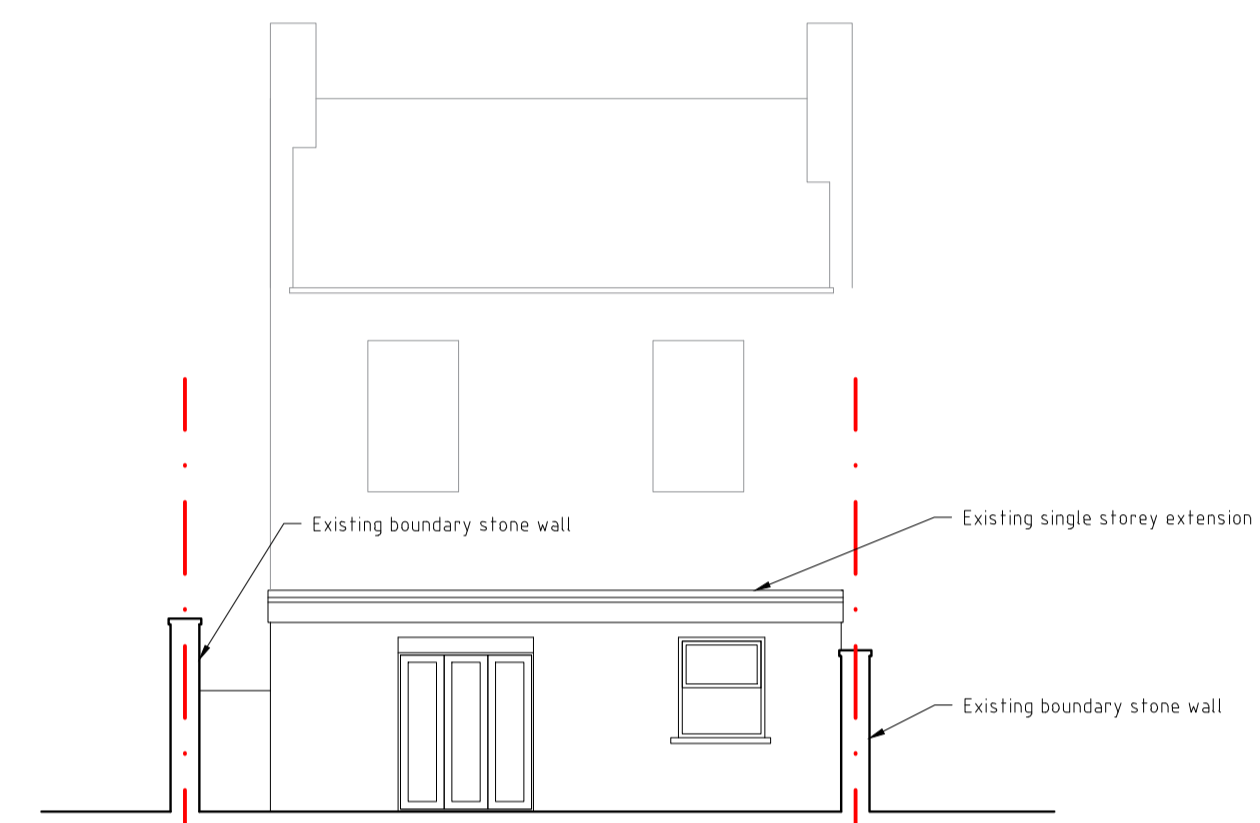
04 North West Elevation As Existing 1:100 @ A1
