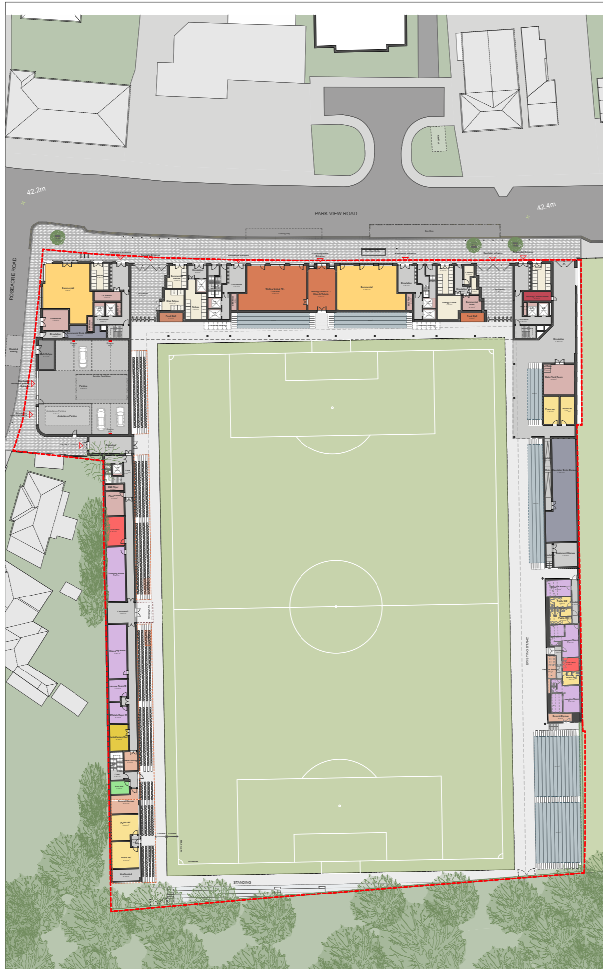
0 Ground Floor Plan 1:500 0 10 20 50
