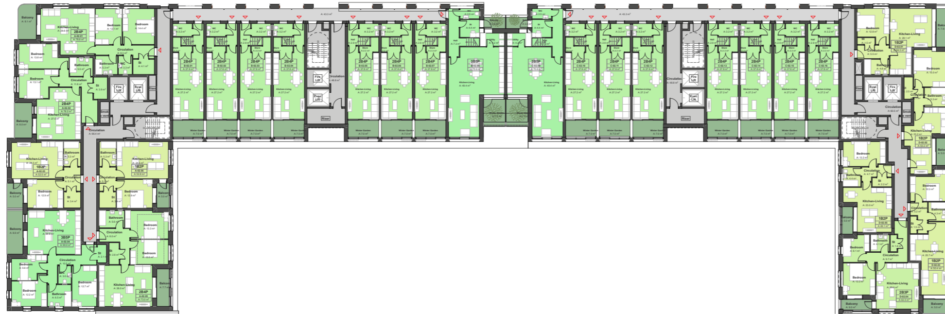
1 Level 02 Floor Plan 1:200
