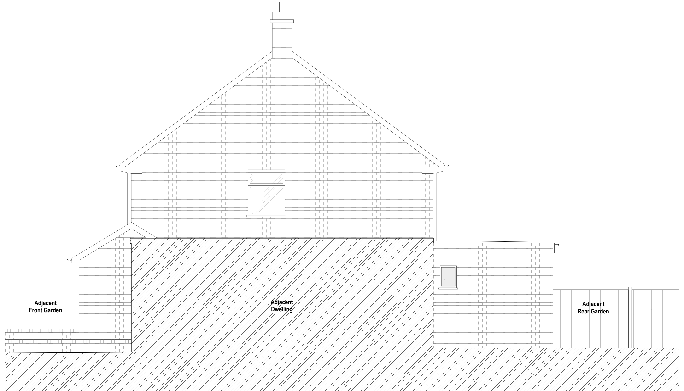
Existing Side Elevation (South) 1:50
