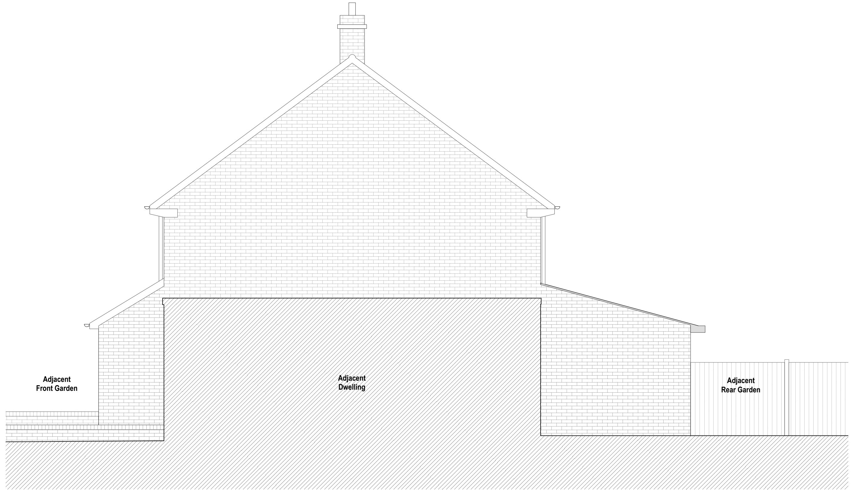
Proposed Side Elevation (South) 1:50
