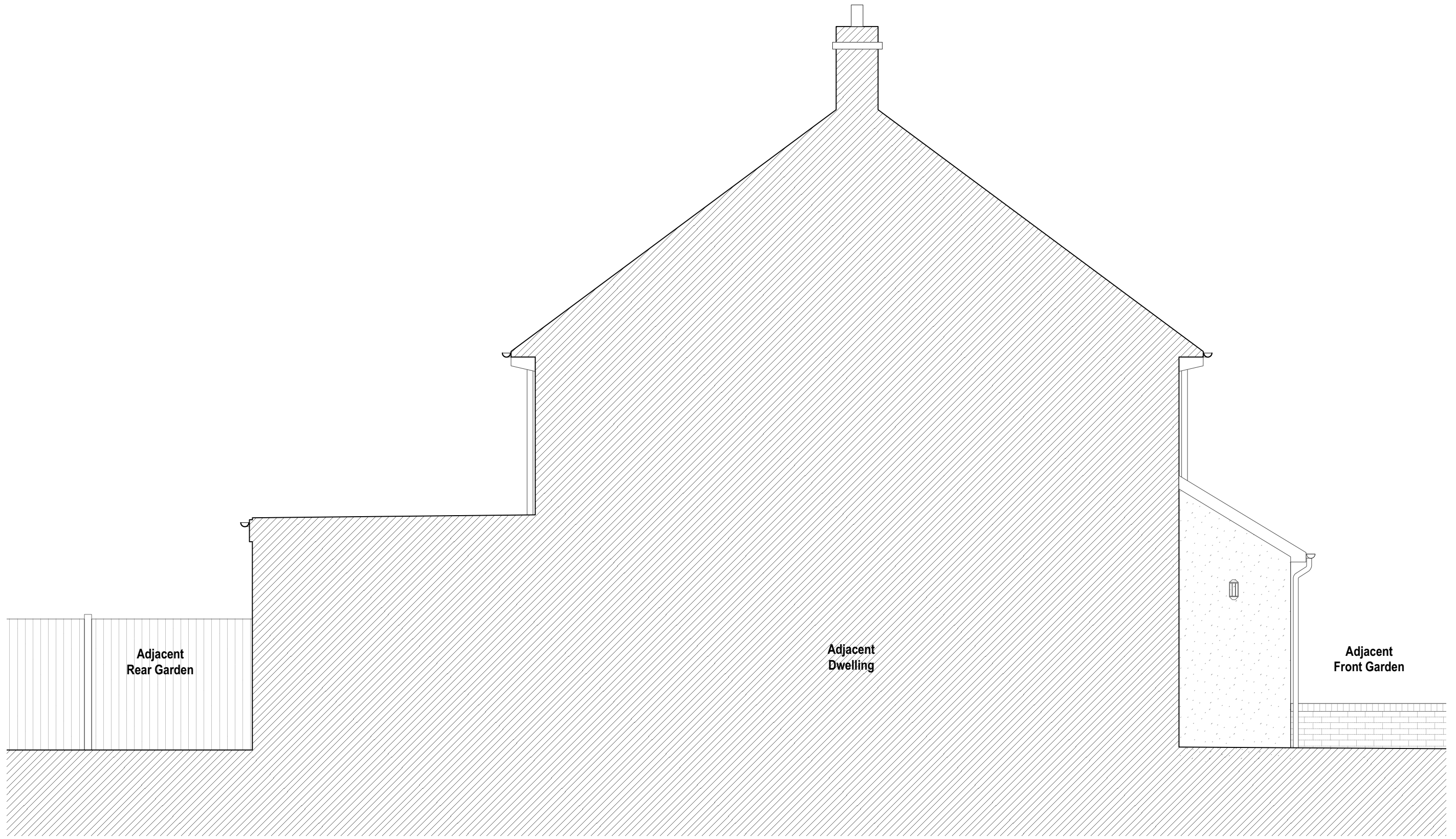
Existing Side Elevation (North) 1:50
