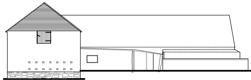
Rear Elevation
