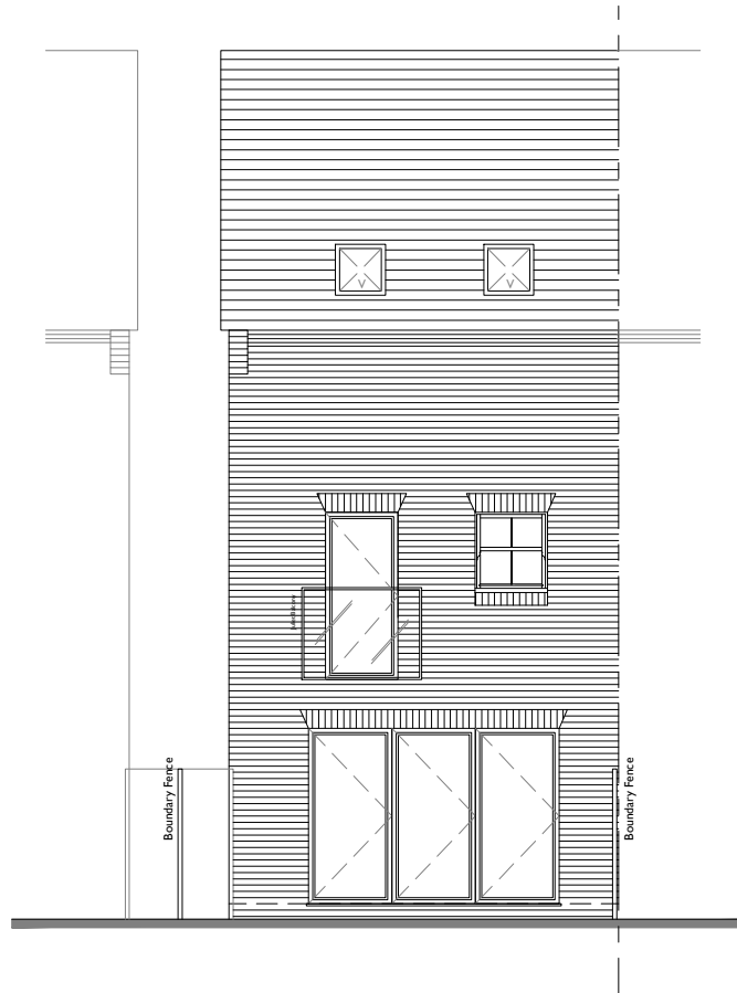
Rear Elevation
