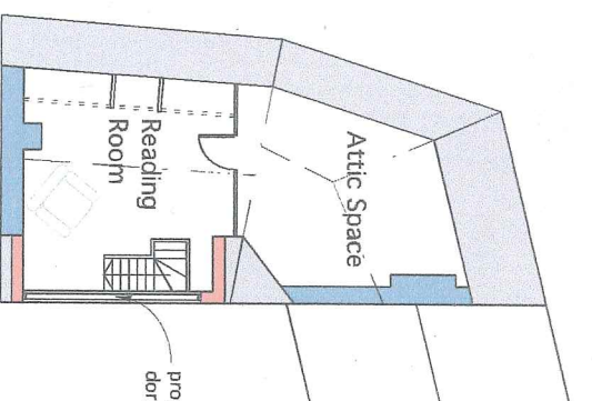
Existing Attic Plan
