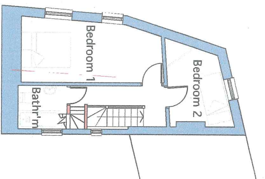
Existing First Floor Plan
