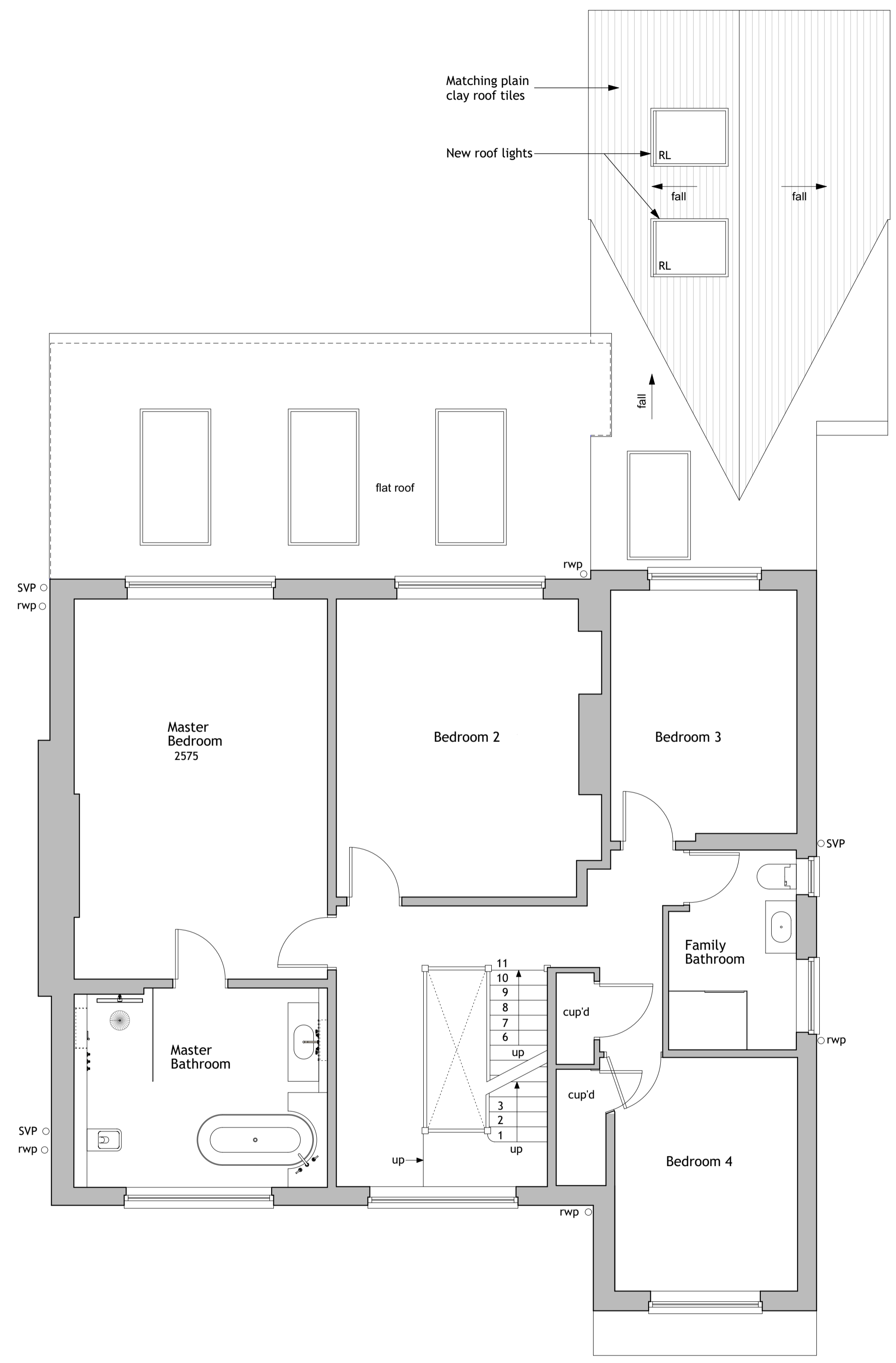
02 First Floor Layout Scale: 1:50
