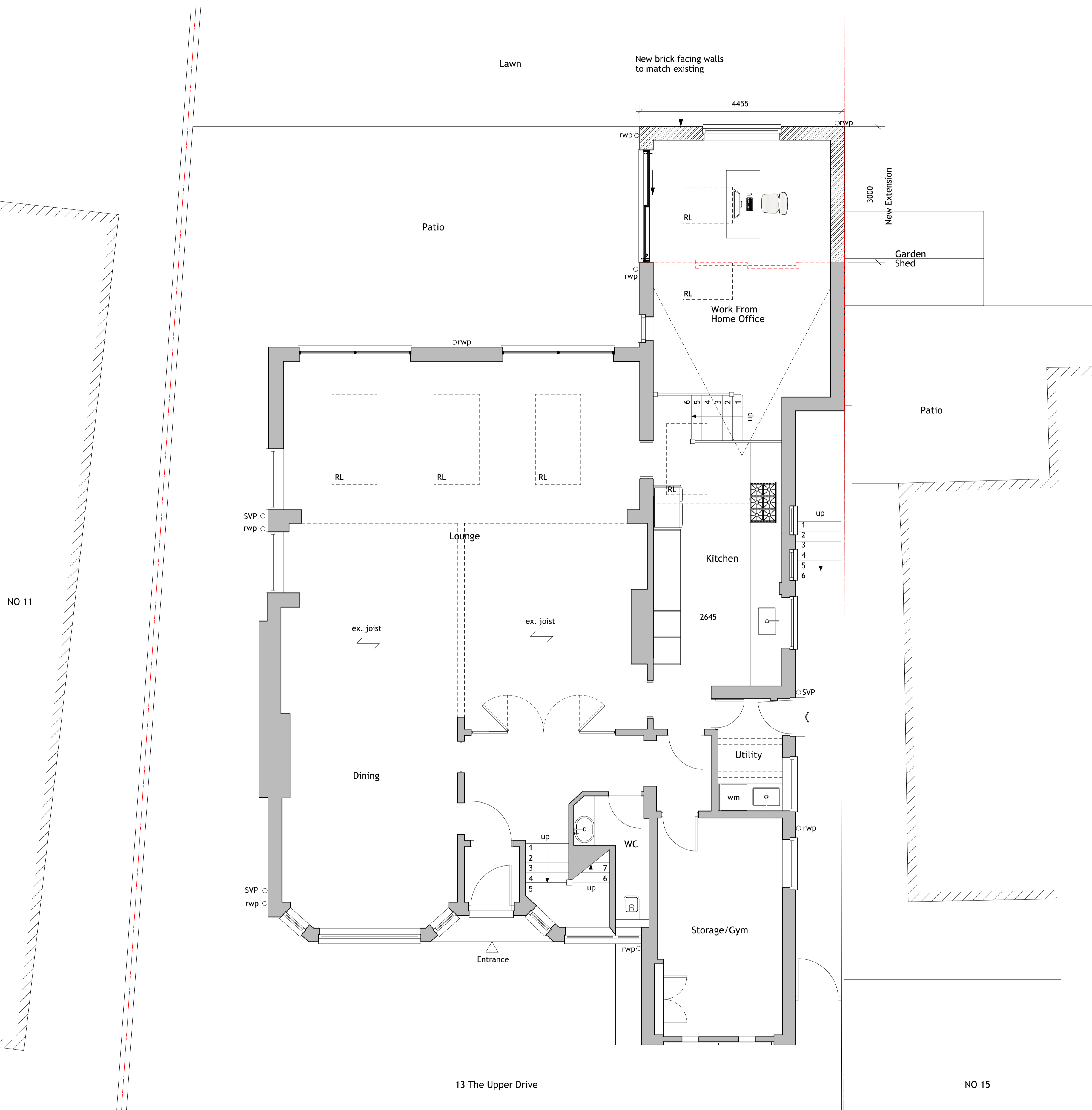
01 Ground Floor Layout Scale: 1:50
