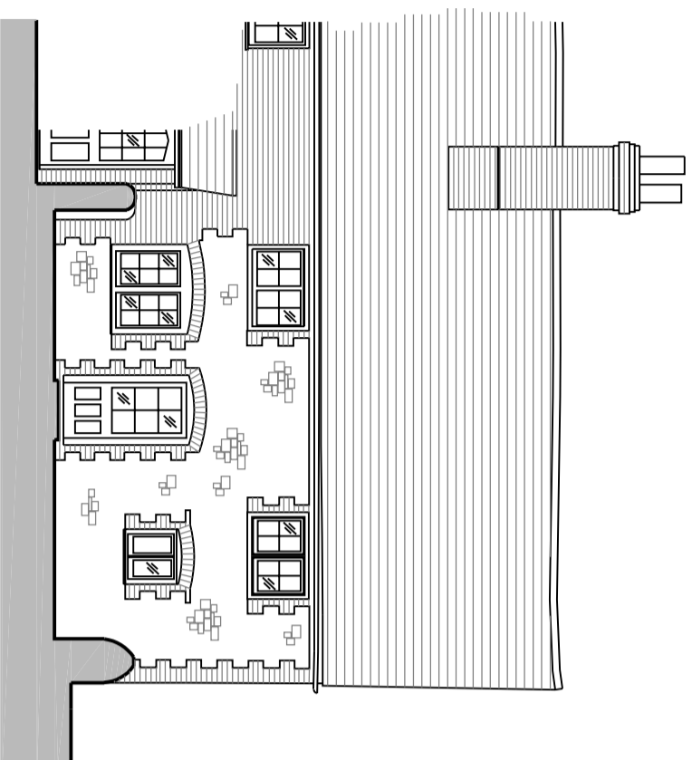
EAST ELEVATION
