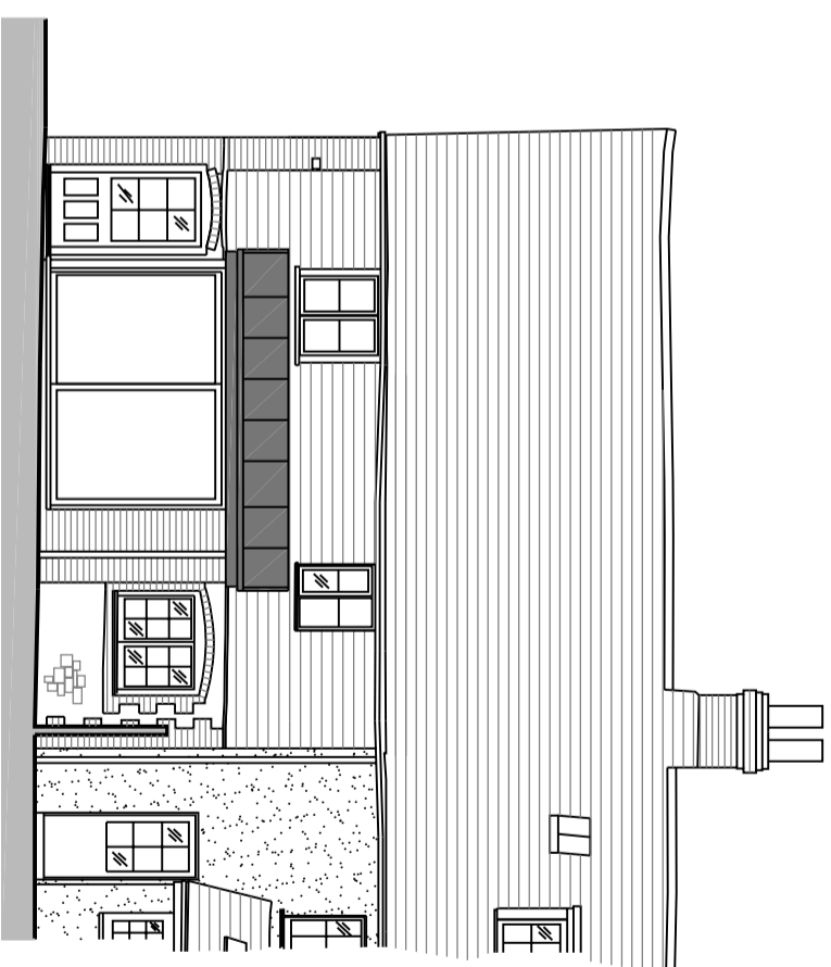
WEST ELEVATION
