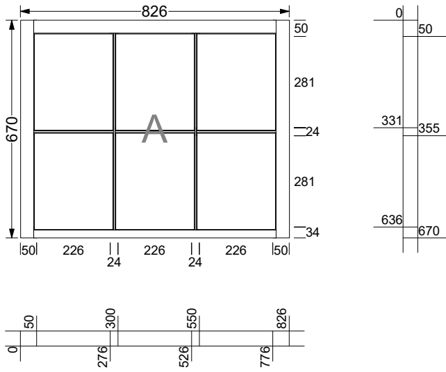
W2 Top sliding sash
