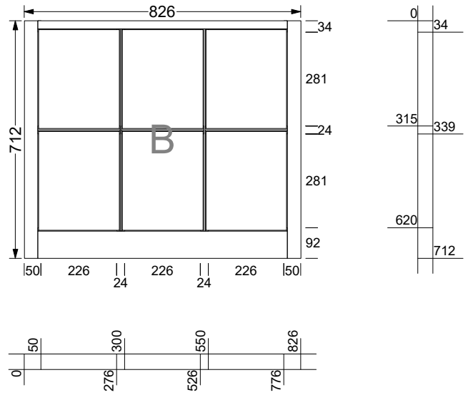
W3 Bottom sliding sash
