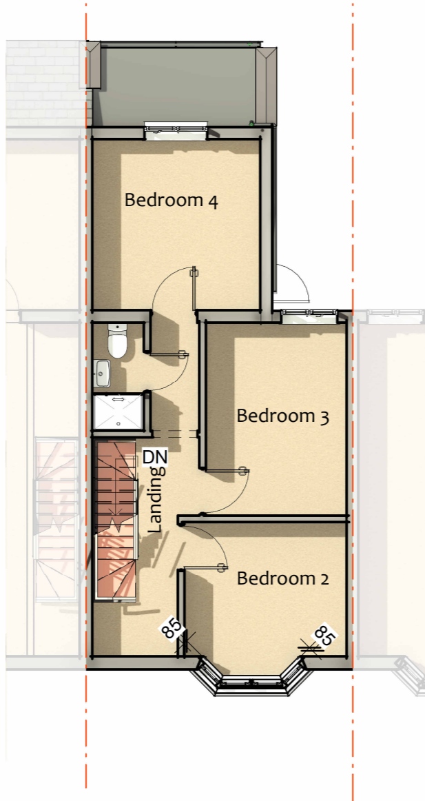
FF EX. FIRST FLR SCALE 1 : 100
