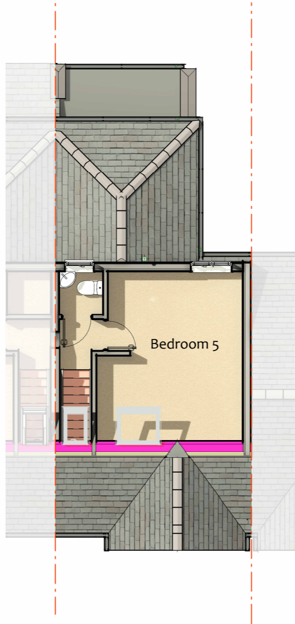
SF EX. SECOND FLR SCALE 1 : 100
