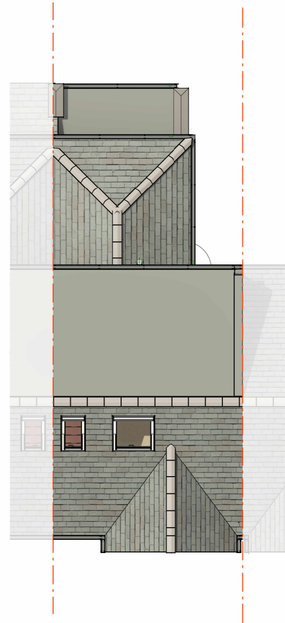
RP EX. ROOF PLAN. SCALE 1 : 100
