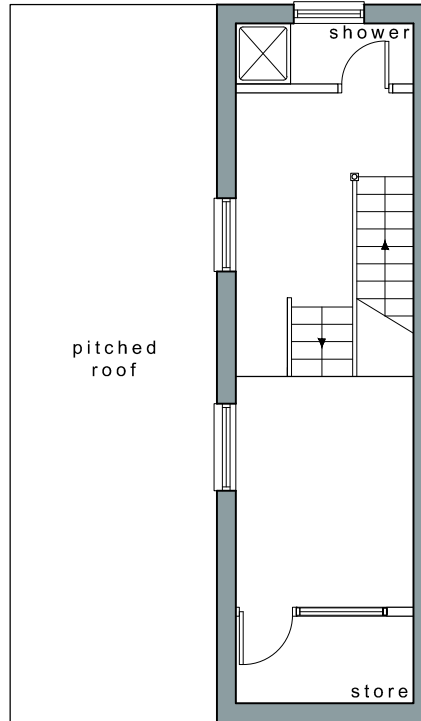
existing upper floor plan scale 1:100
