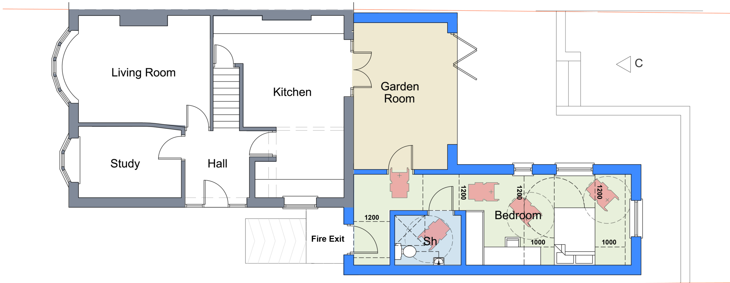
Proposed Rear Extension to included DDA requirements
