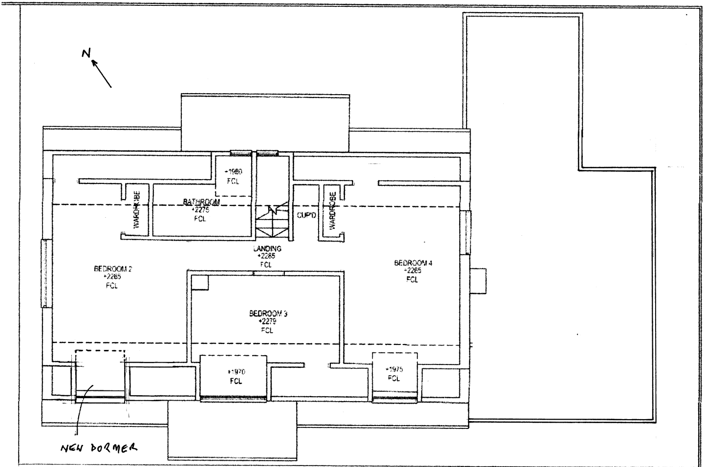
FIRST FLOOR - PROPOSED FLOOR PLAN
