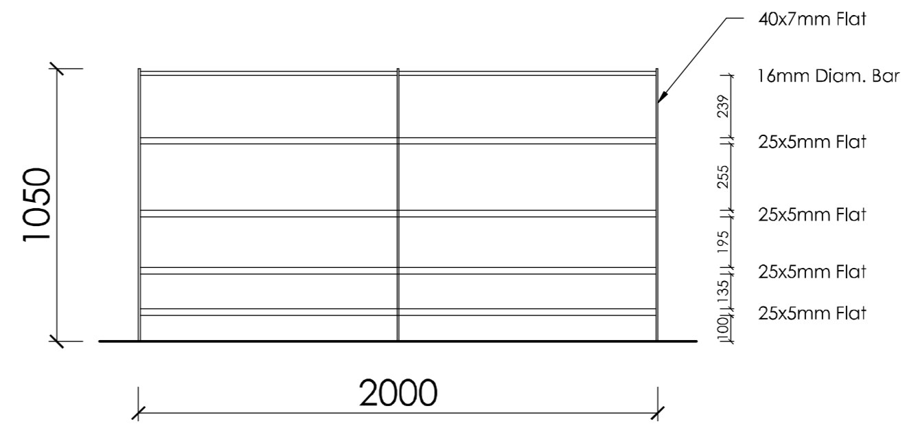
Iron Estate Railings Panels Elevation 1:20
