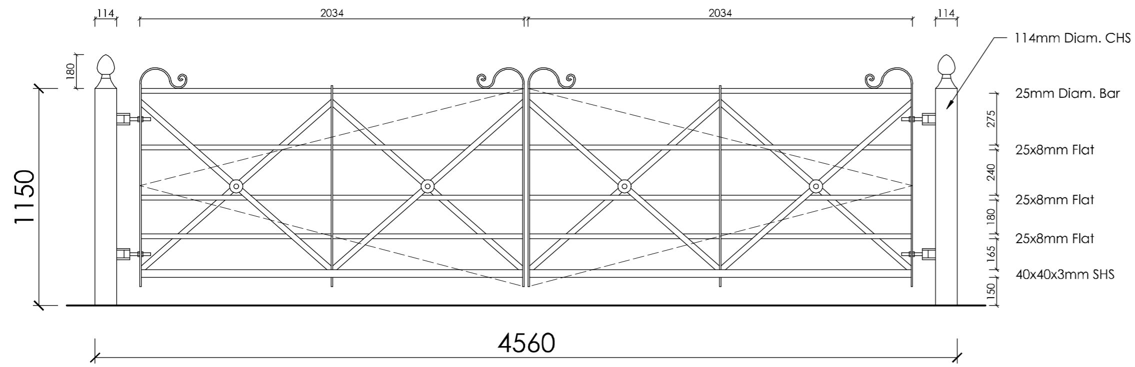
Iron Gates Elevation 1:20
