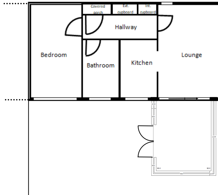
GROUND FLOOR 1:100
