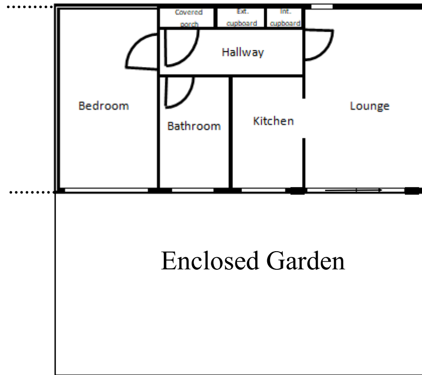
GROUND FLOOR 1:100
