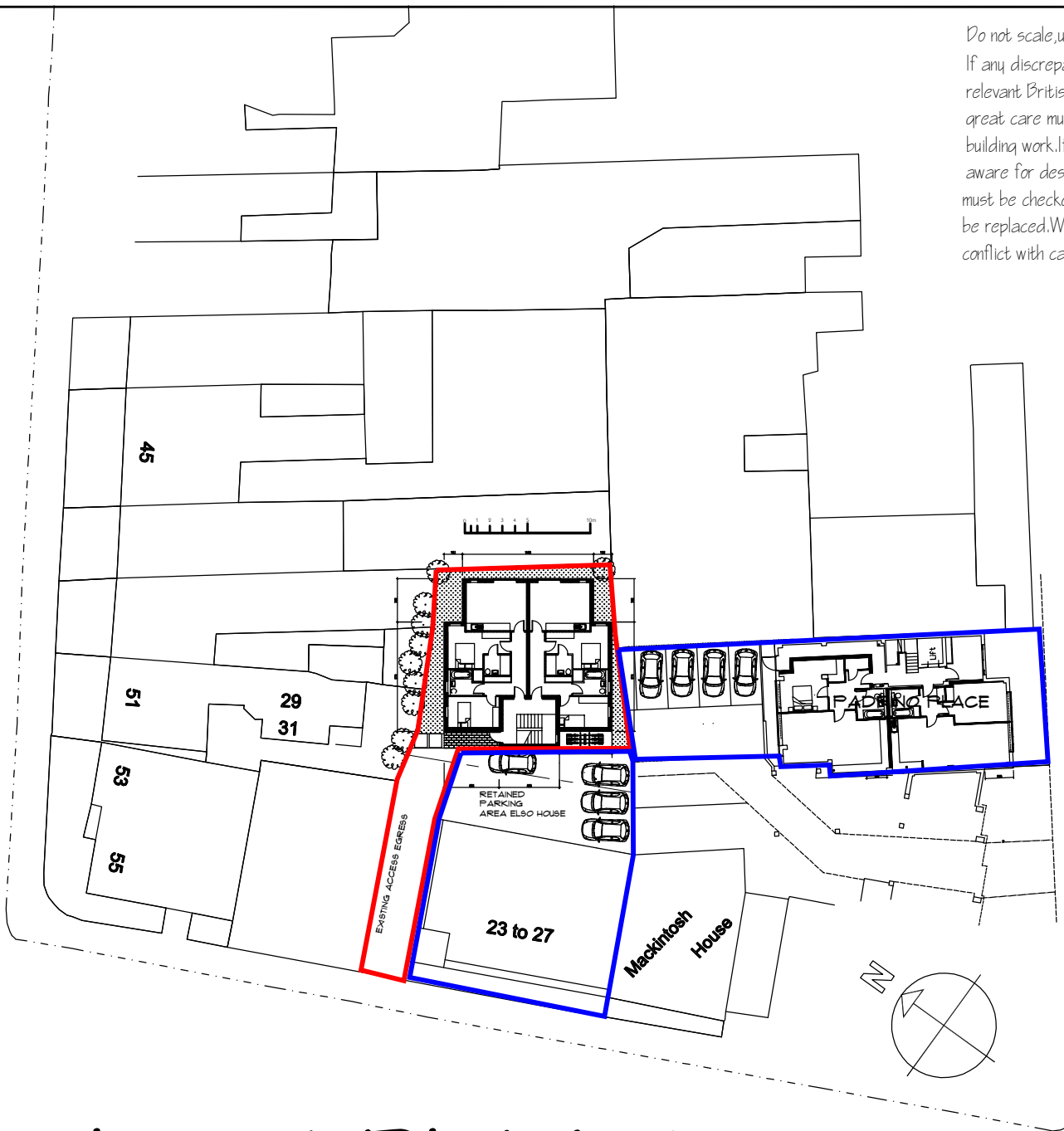
BLOCK PLAN 1:500
