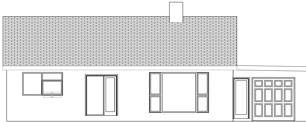
E-01 East Elevation 1:100
