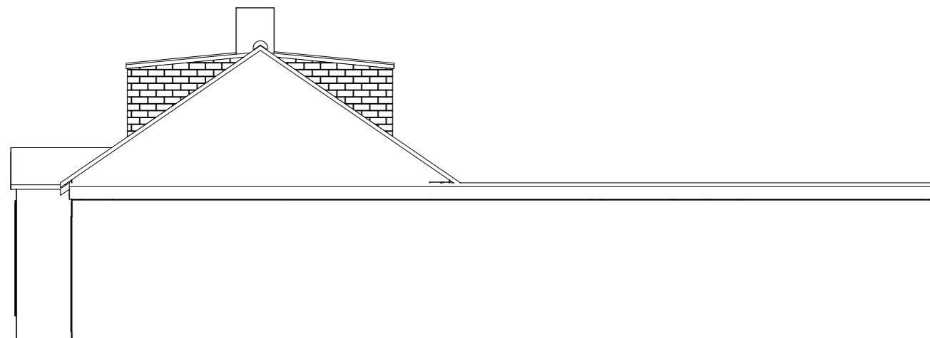
E-03 North Elevation 1:100
