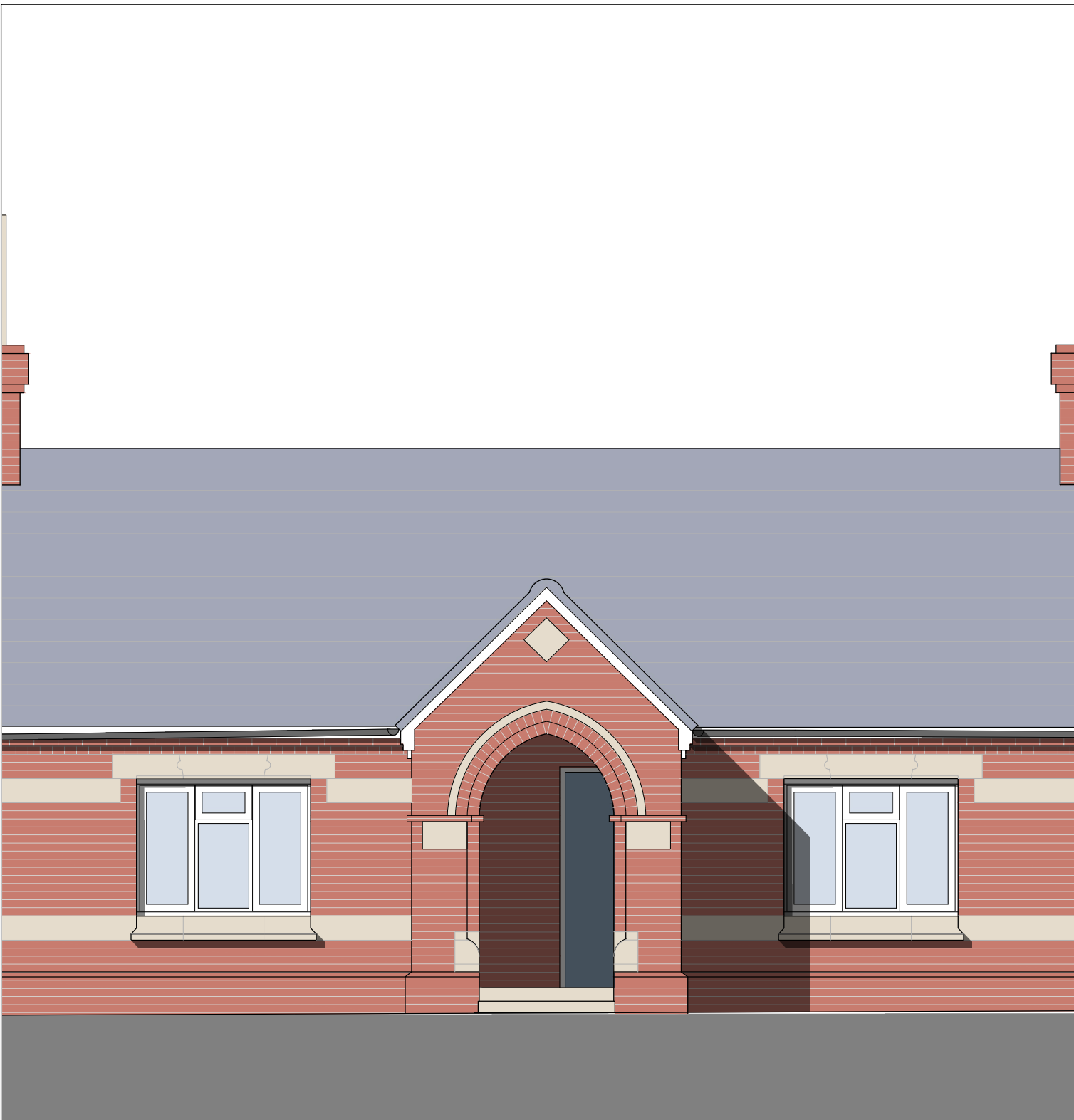
Front Elevation
