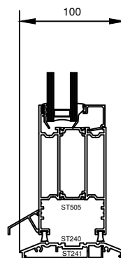
07 DOOR THRESHOLD DETAIL
