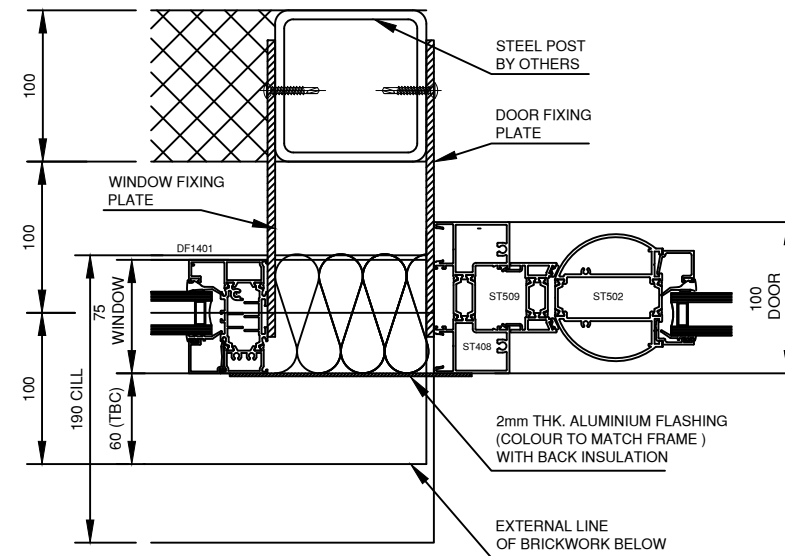
04 WINDOW, DOOR & STEEL POST JUNCTION DETAIL
