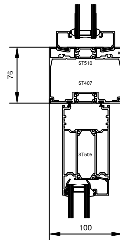
06 DOOR HEAD DETAIL
