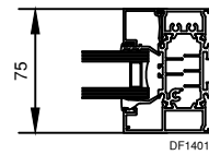
03 WINDOW JAMB DETAIL
