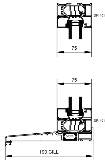
01 WINDOW HEAD DETAIL
