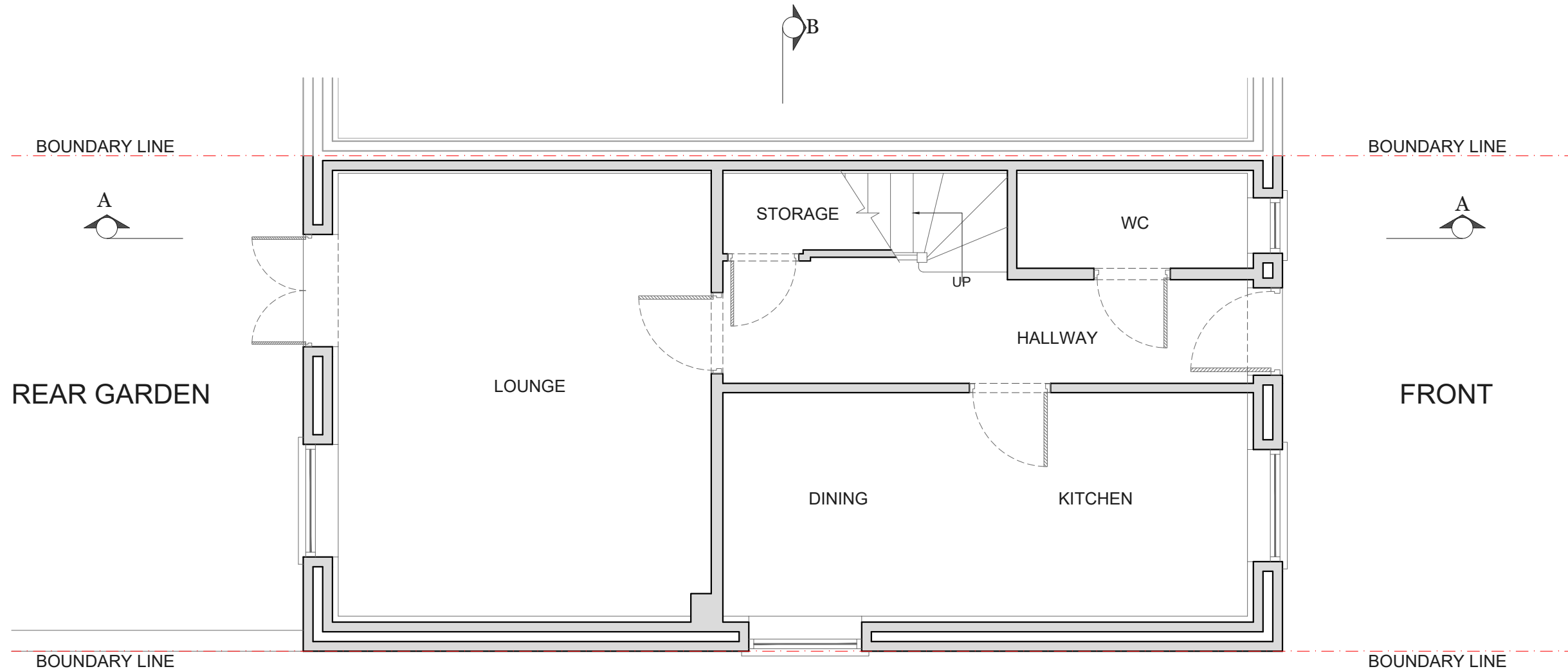
EXISTING GROUND FLOOR PLAN SCALE 1:50
