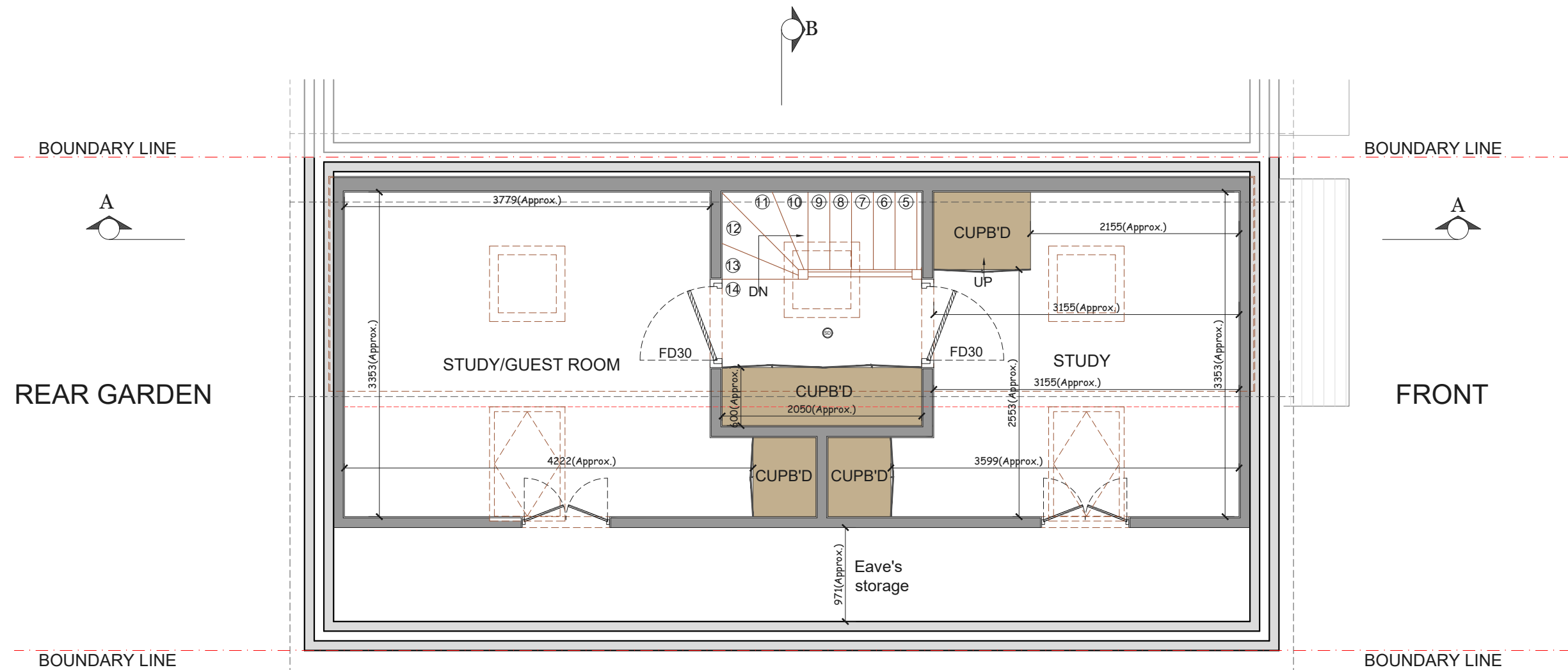
PROPOSED LOFT FLOOR PLAN SCALE 1:100
