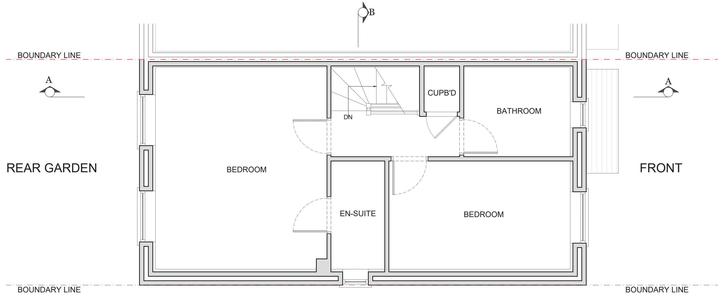
EXISTING FIRST FLOOR PLAN SCALE 1:100
