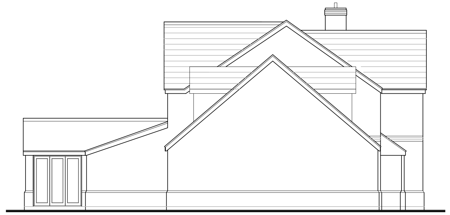
SIDE ELEVATION
