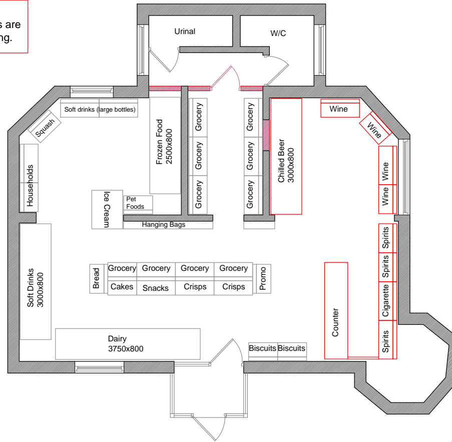
PROPOSED FLOOR PLAN Scale 1:100
