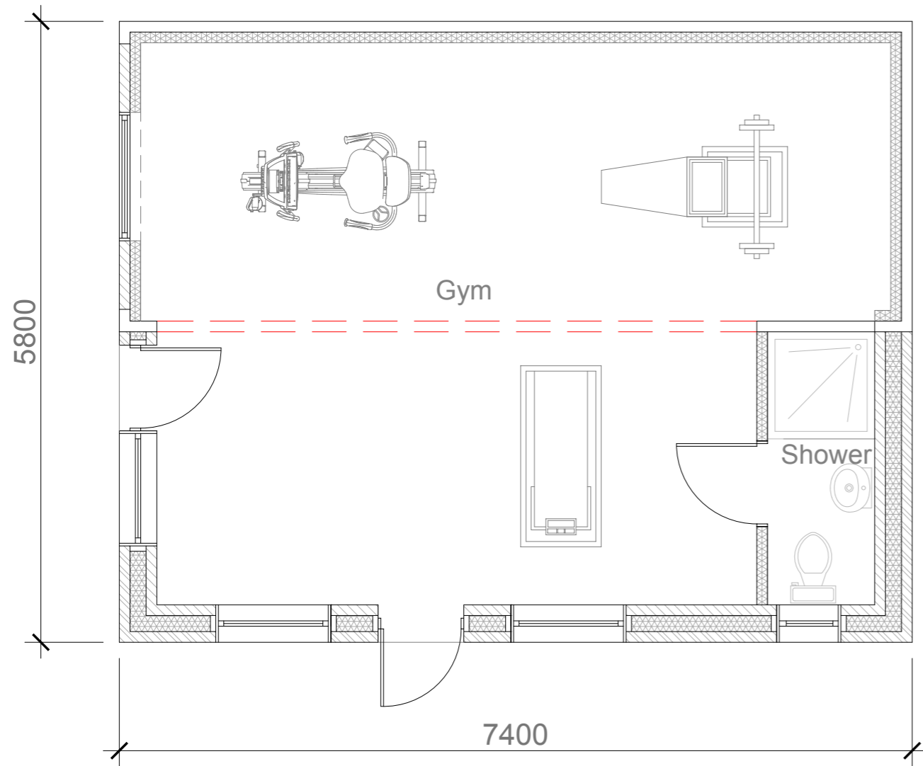
PROPOSED OUTBUILDING PLAN 1:50
