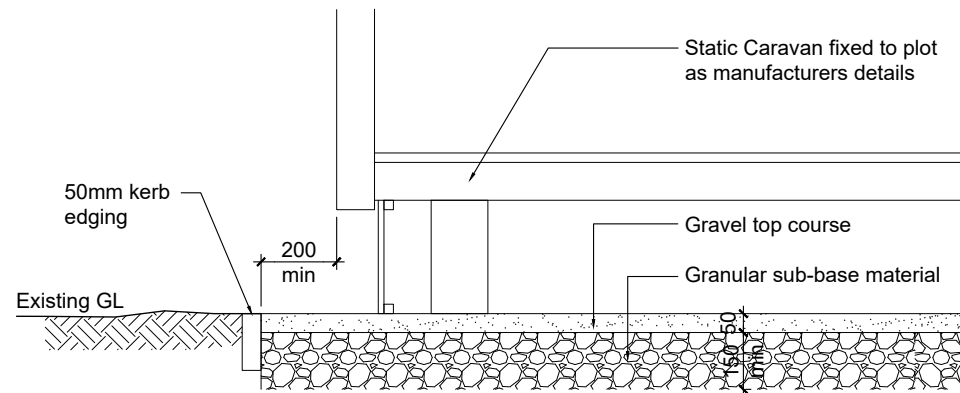
DETAIL 1 Static Caravan Base Details
