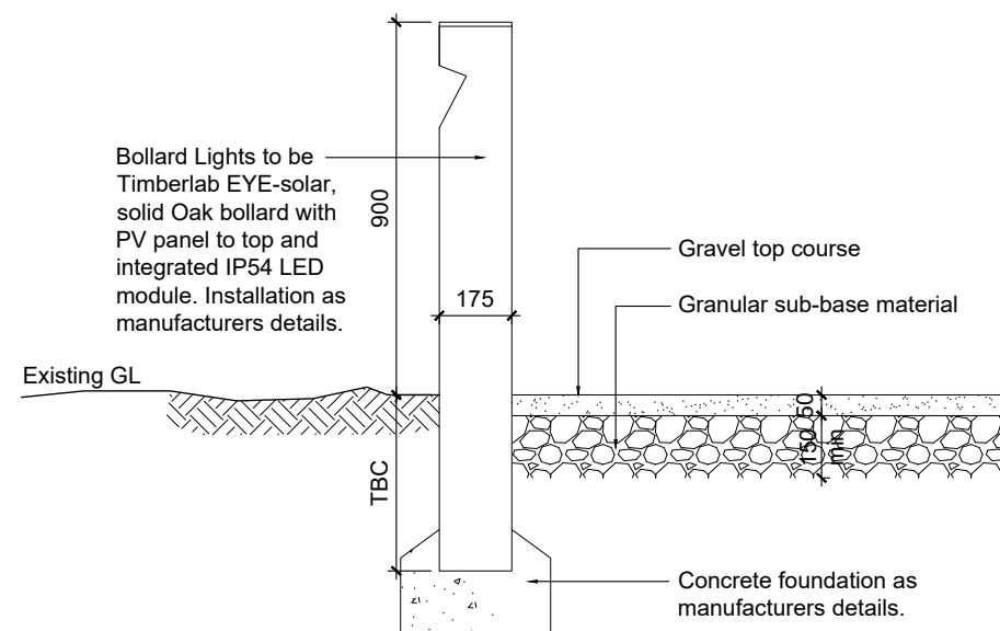
DETAIL 2 External Light Details
