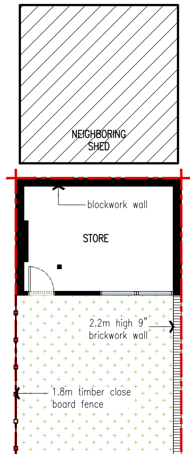
[01] EXISTING FLOOR PLAN 1:100
