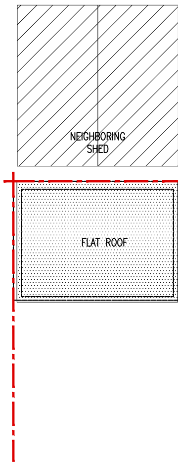
[02] EXISTING ROOF PLAN 1:100
