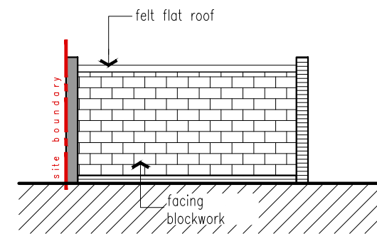
[05] EXISTING WEST ELEVATION 1:100
