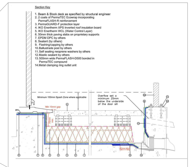
DECK STANDARD DETAIL - NTS
