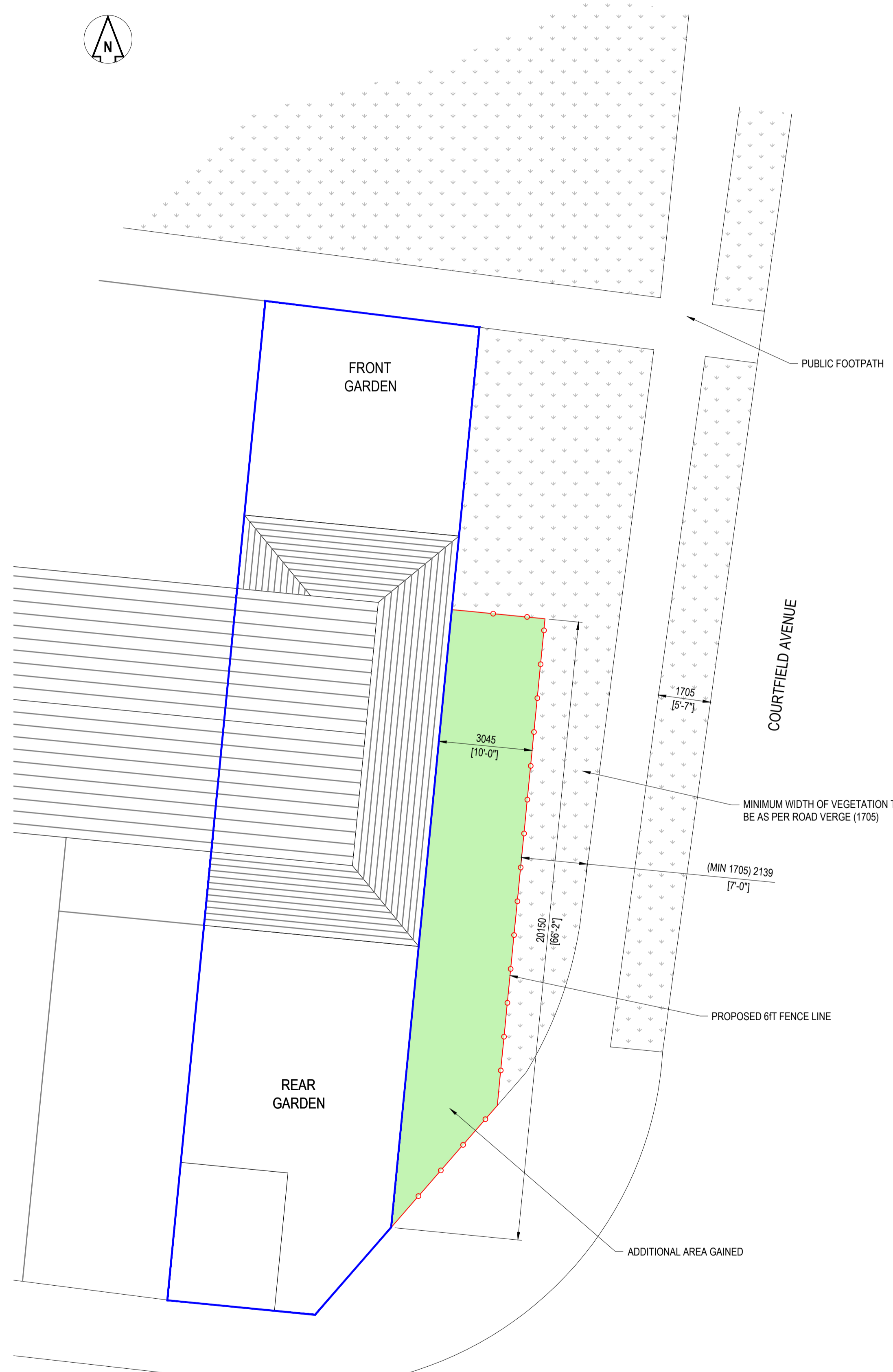
PROPOSED PLAN SCALE 1:100
