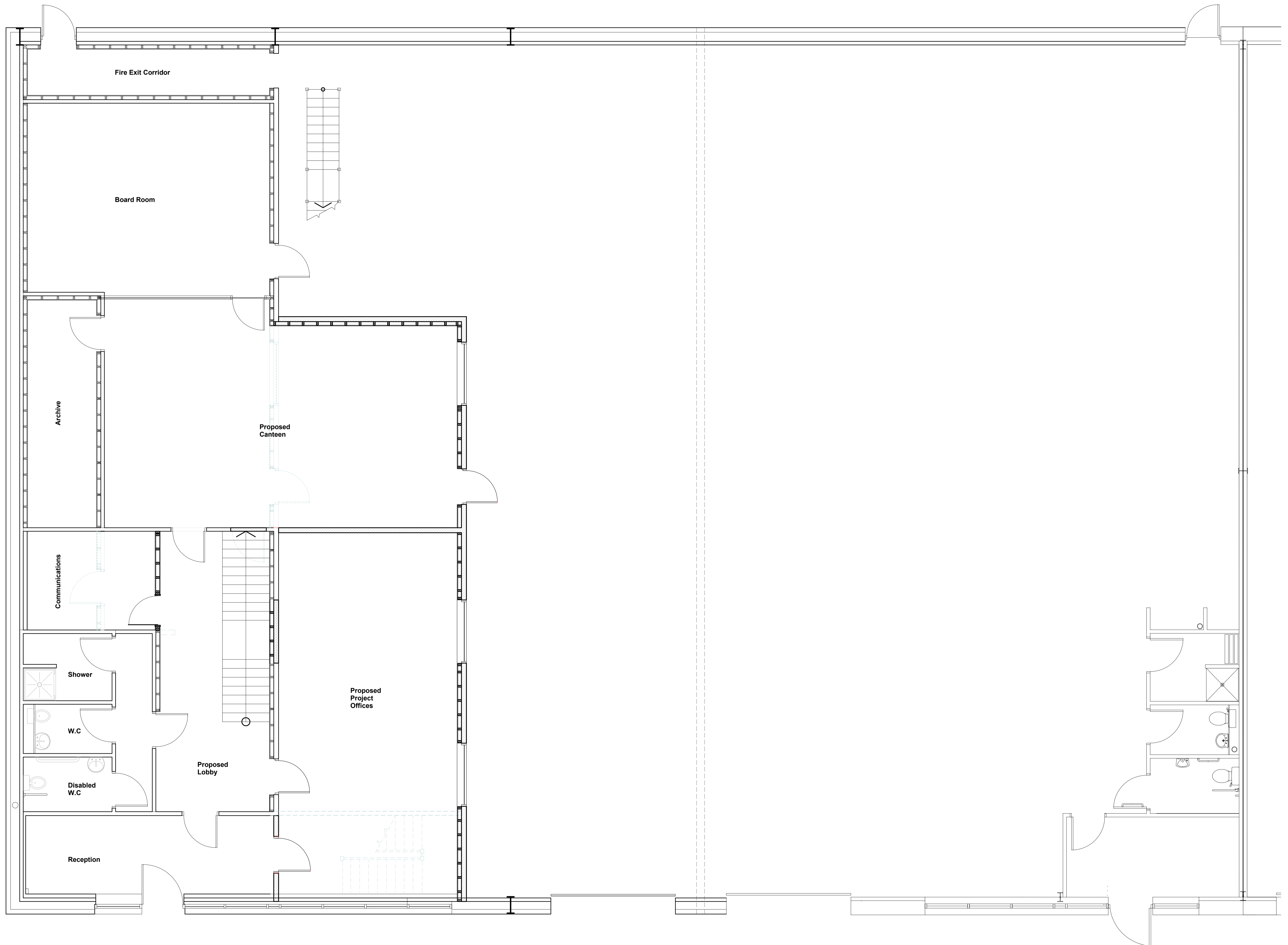
Proposed Ground Floor Plan - 1/50
