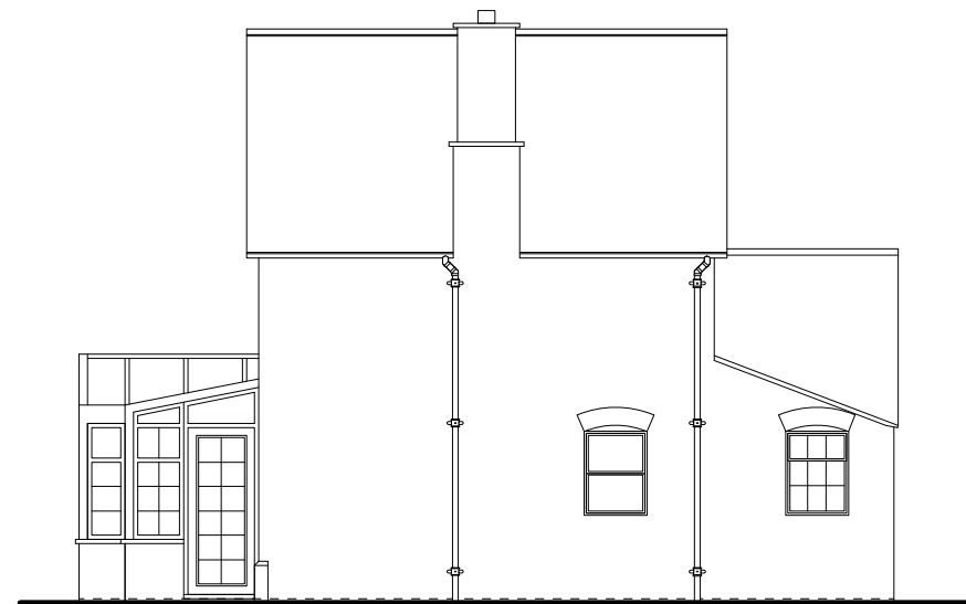
NORTH ELEVATION
