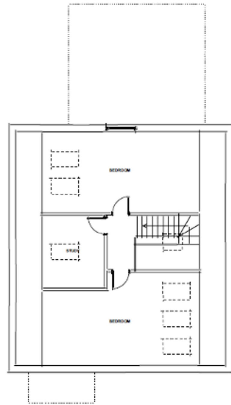
EXISTING SF PLAN
