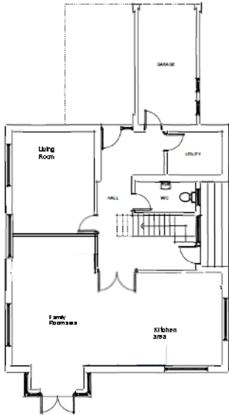
EXISTING GF PLAN
