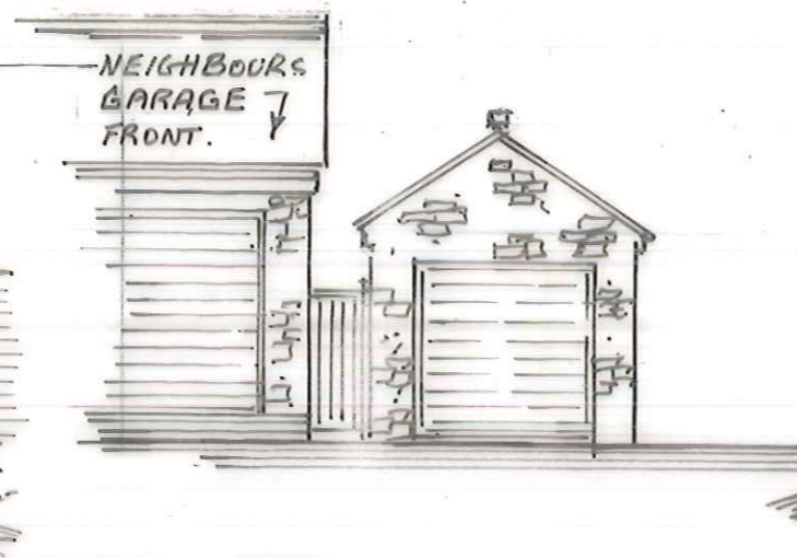
FRONT EL (EAST)
