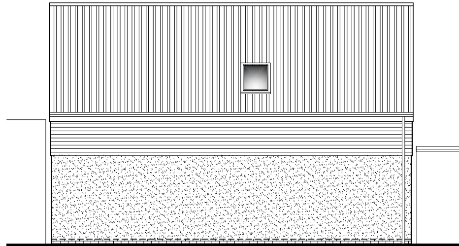
PROPOSED WEST ELEVATION SCALE - 1:100
