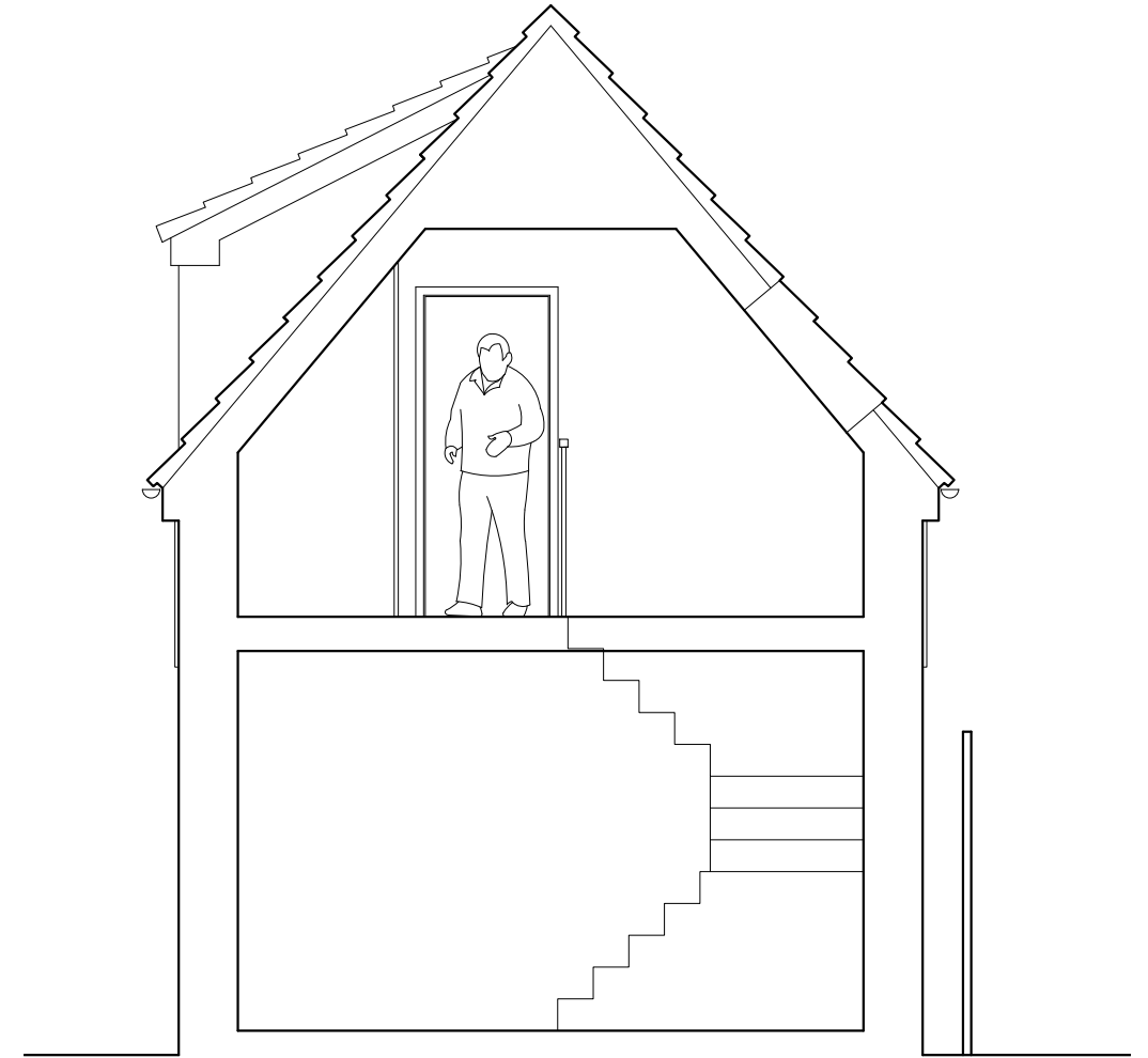
INDICATIVE SECTION SCALE - 1:50
