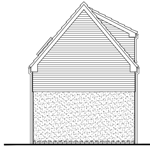
PROPOSED SOUTH ELEVATION SCALE - 1:100
