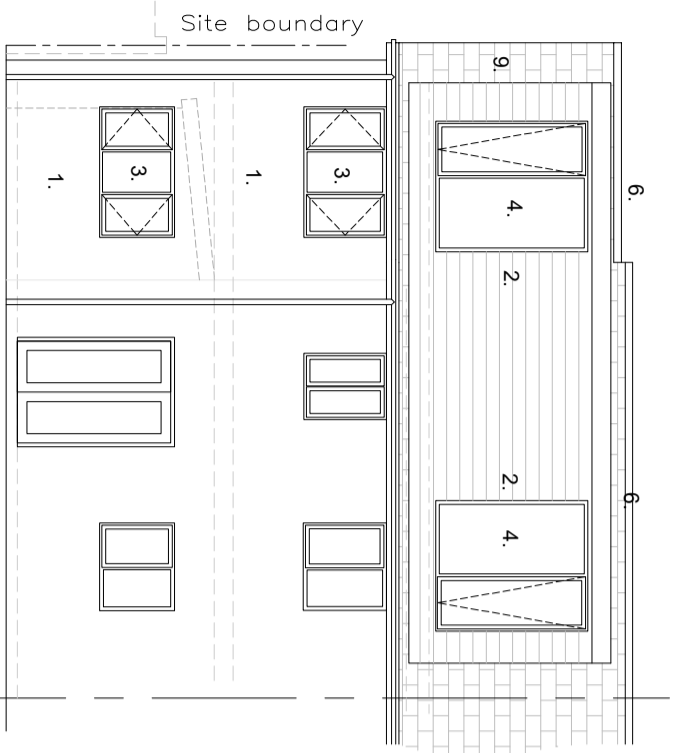
South Elevation Proposed
