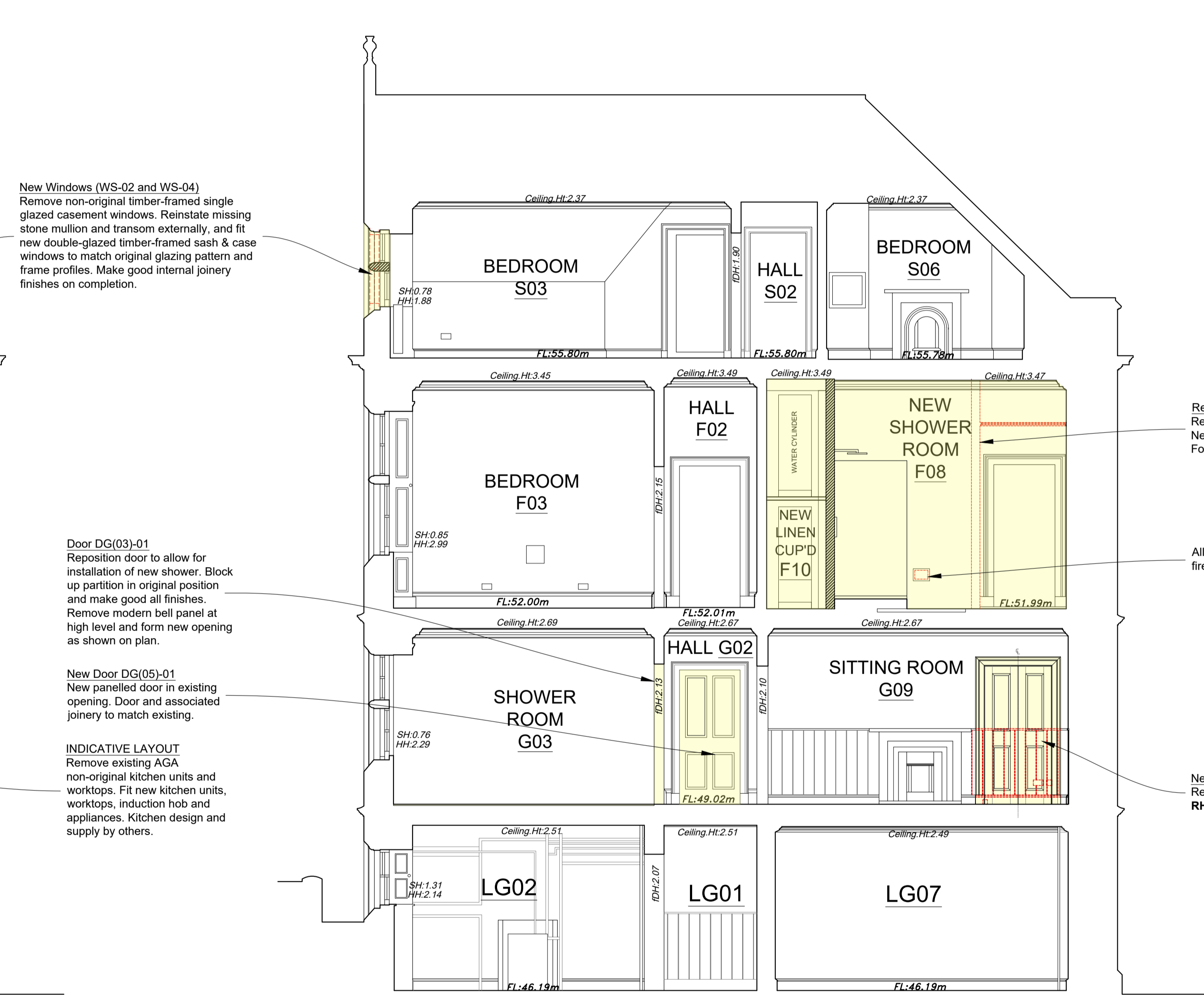
Section BB as Proposed Scale 1:50 @ A1
