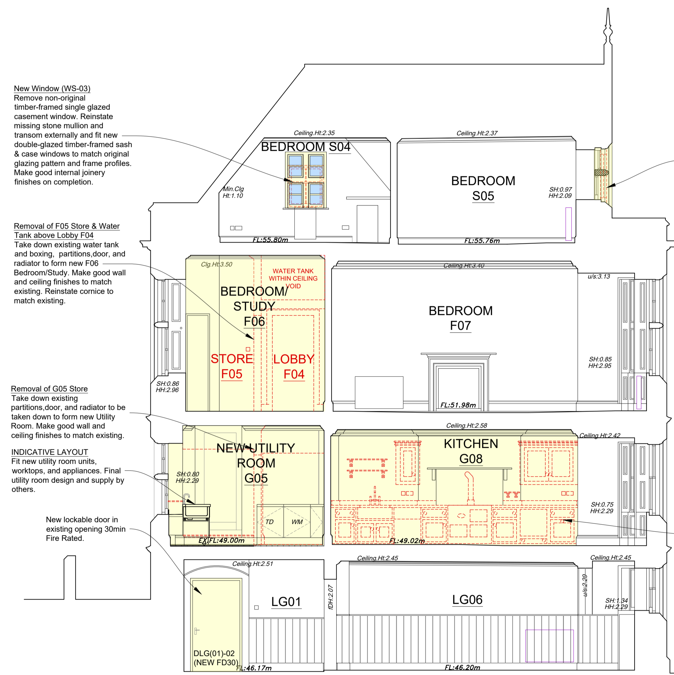
Section AA as Proposed Scale 1:50 @ A1
