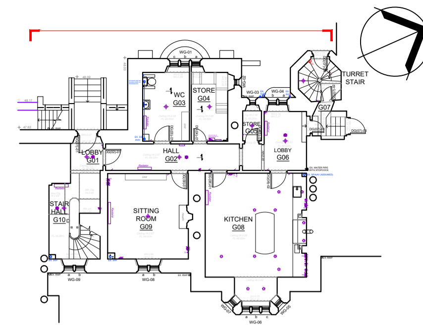
Key Plan Scale 1:200 @ A1
